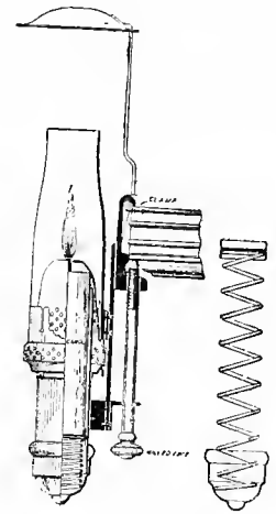
Figs. 3248-3249. BRACKET EMERGENCY CANDLE LAMP, PULLMAN'S PATERN.
